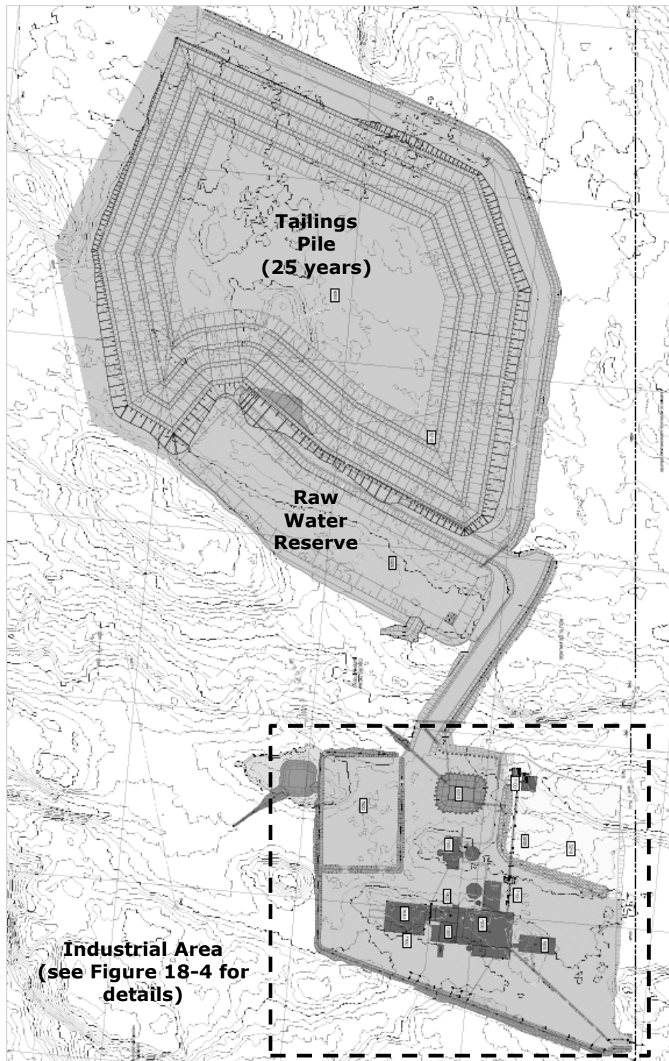
Figure 18-3 - Baie-Comeau Site Plot Plan - General
