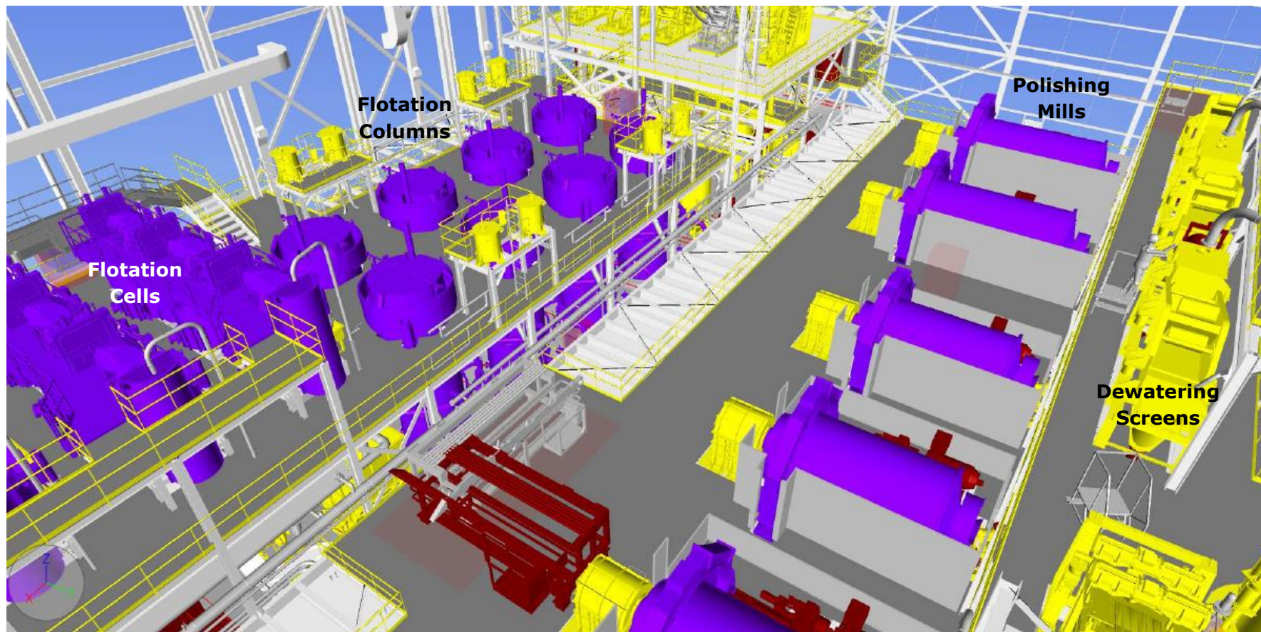
Figure 17-3 - Area 04 – Polishing Grinding and Cleaning Flotation
