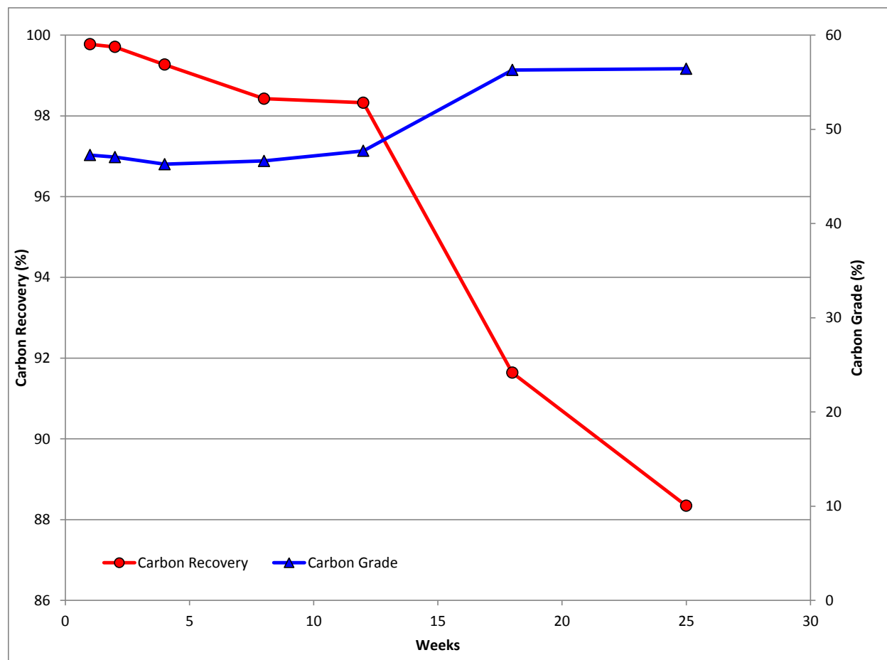
Figure 13-9 - Rougher and Scavenger Concentrates Grade and Recovery 1
