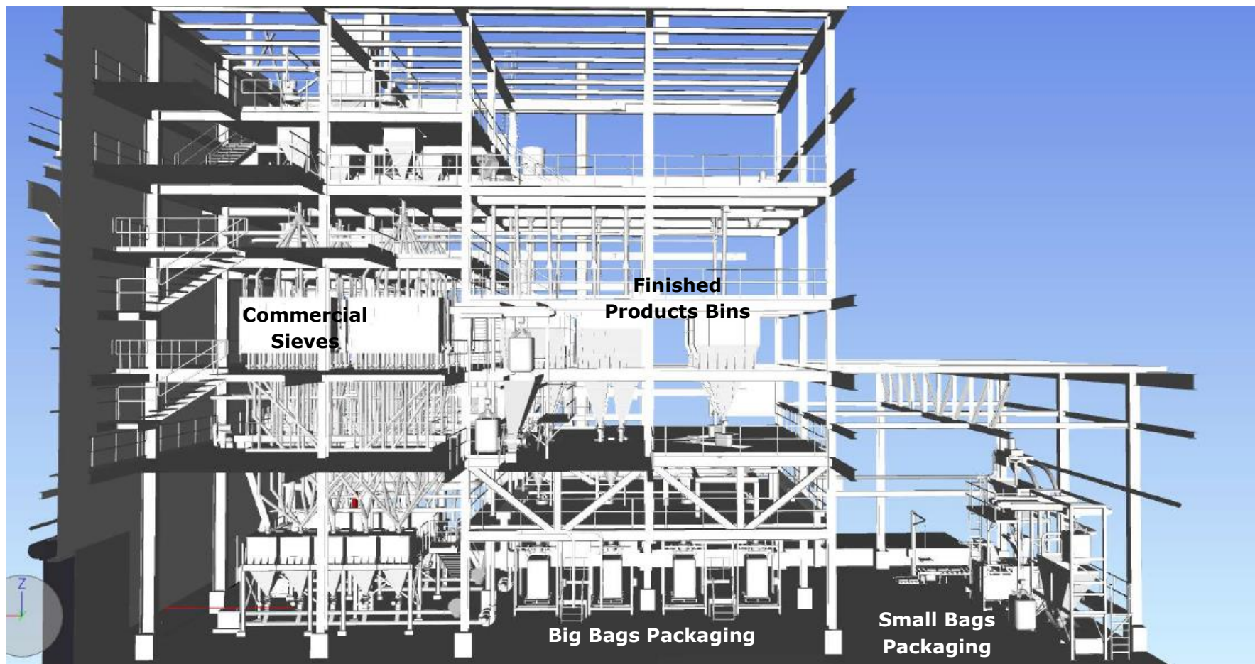
Figure 17-6 - Area 06 – Commercial Sieving and Area 07 – Concentrate Bagging
