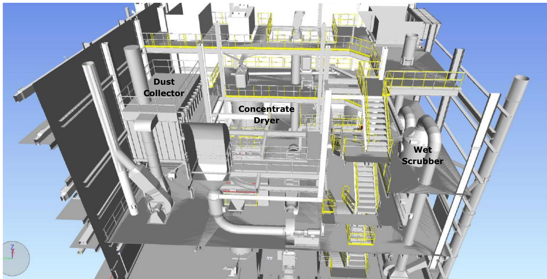
Figure 17-5 - Area 05 – Cut-out of the Dryer and Scrubber
