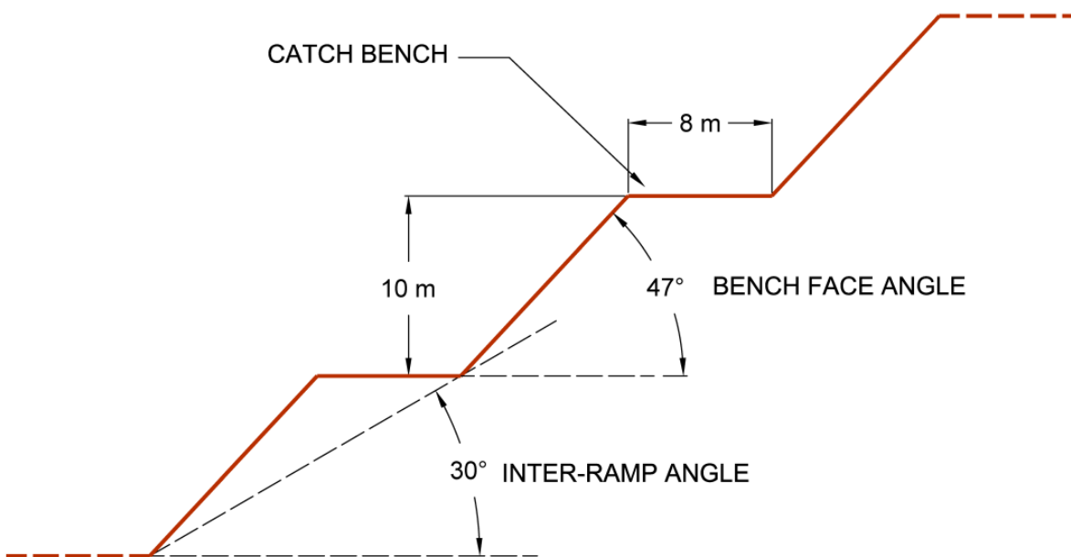
Figure 15-4 - Pit Wall Configuration
