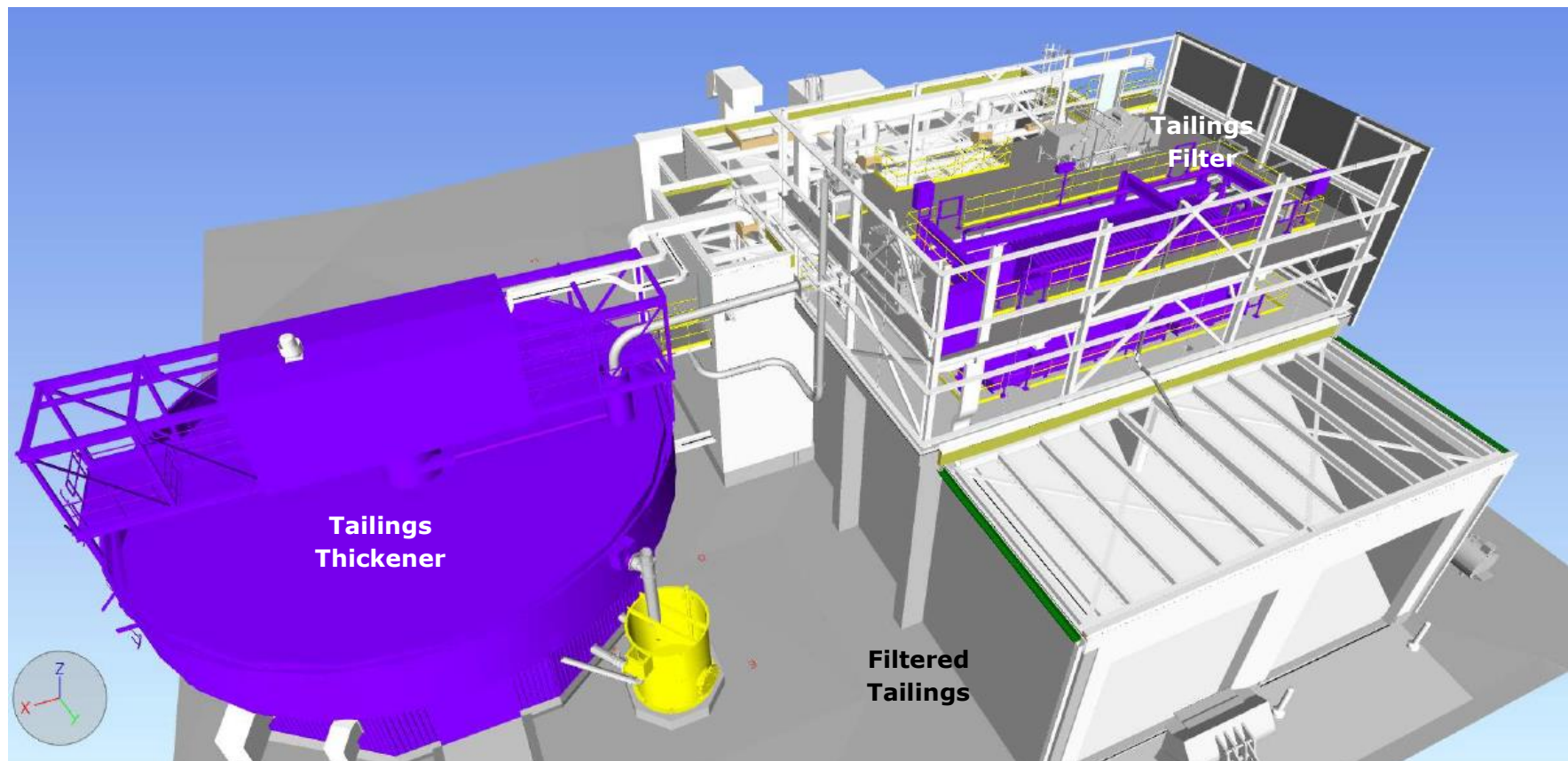
Figure 17-7 - Area 08 - Tailings Filtration
