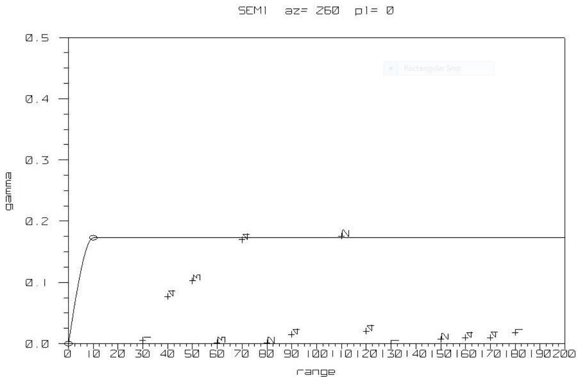
Figure 14.4: Drilling Semivariogram
