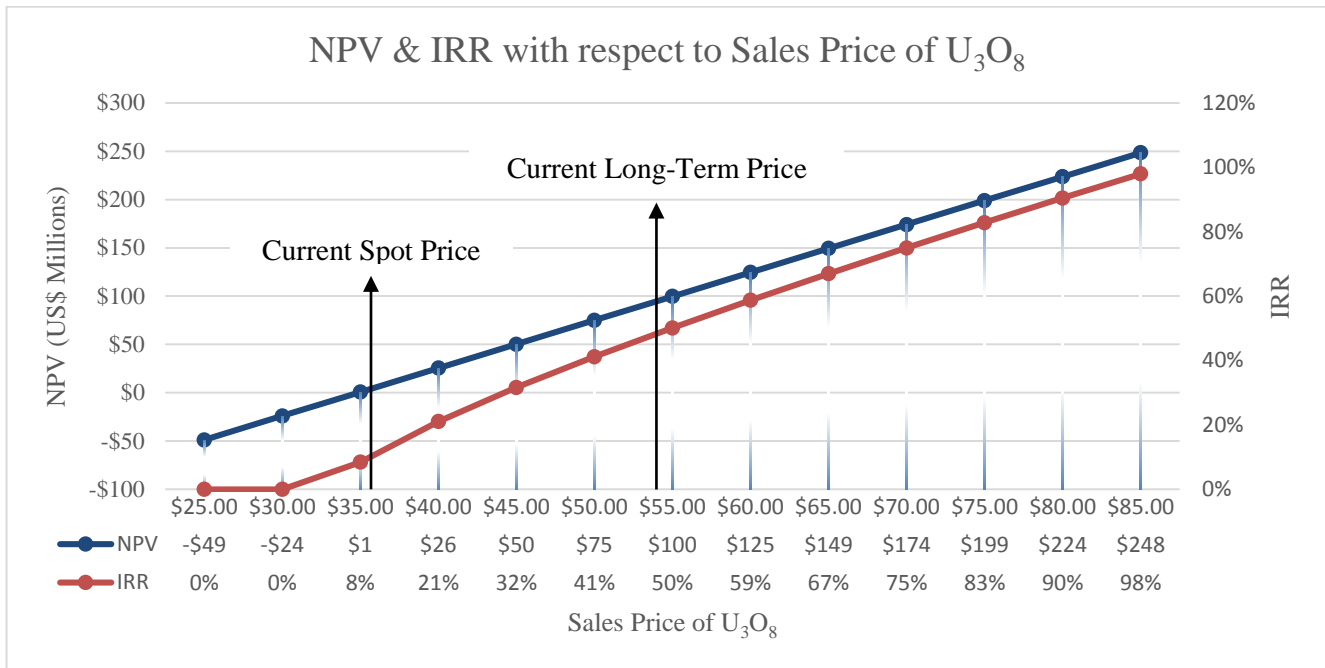
Figure 22.1: NPV & IRR v. Uranium Price (Pre-U.S. Federal Income Tax)
