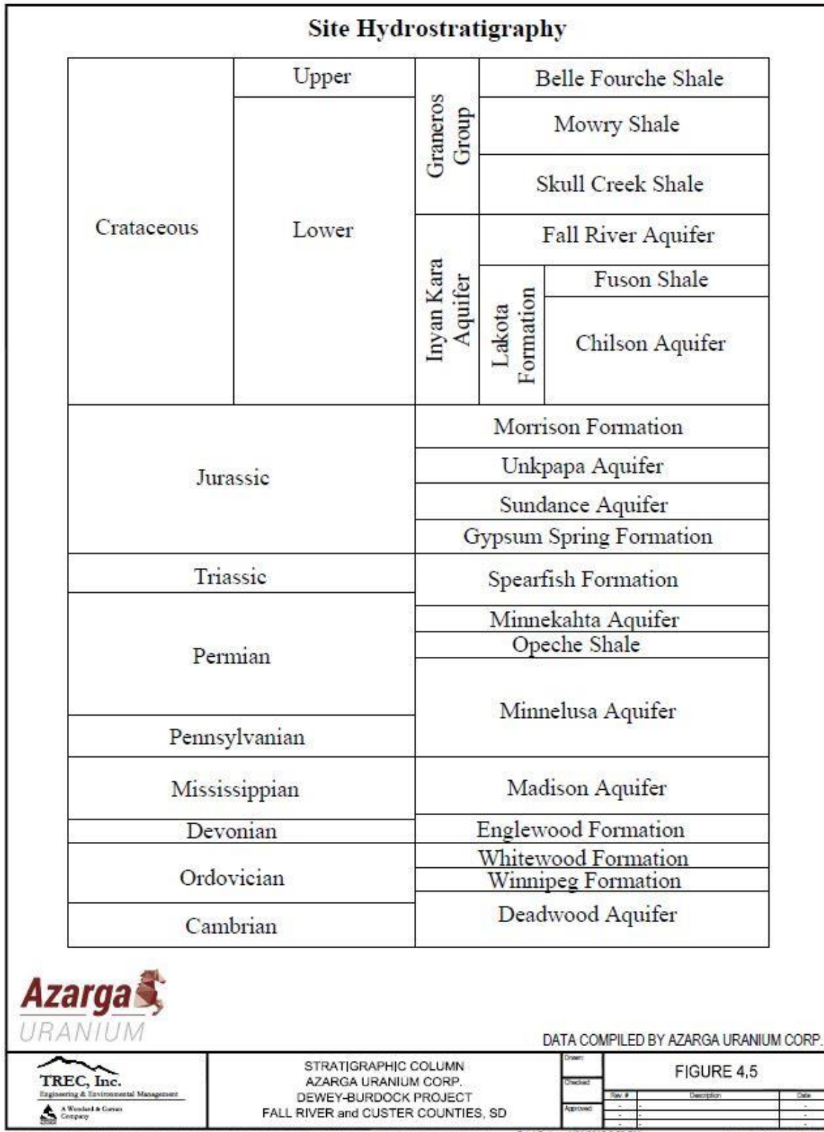
Figure 4.5: Stratigraphic Column
