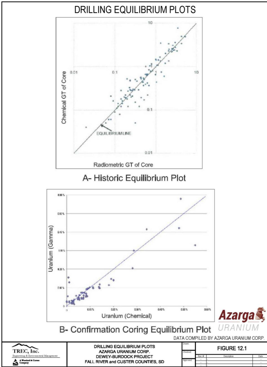
Figure 12.1: Equilibrium Plot
